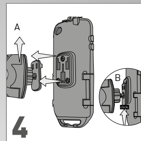
4 Snap the case onto the bracket.
